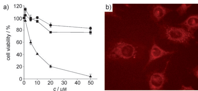
Figure 3. a) Cytotoxicity in HeLa cells by MTT assay for Tat CPP (●), TLD-t (■), and TLD-d (▲). Mean values \pm standard deviation are shown ( n = 3 ). b) Confocal laser scanning microscopy (CLSM) image (400 \times ) of intracellular delivery of Nile red by TLD-t short-length cylindrical micelles. The TLD-t concentration was 10 \mu\text{M} and the amount of encapsulated Nile red was 3 mol% relative to TLD-t. The cells were treated for 3 h.
